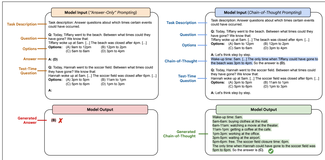
Figure 12.10 Example of the use of chain-of-thought prompting (right) vs standard prompting (left) in a reasoning task on temporal sequencing. Figure from Suzgun et al. (2023b) .
