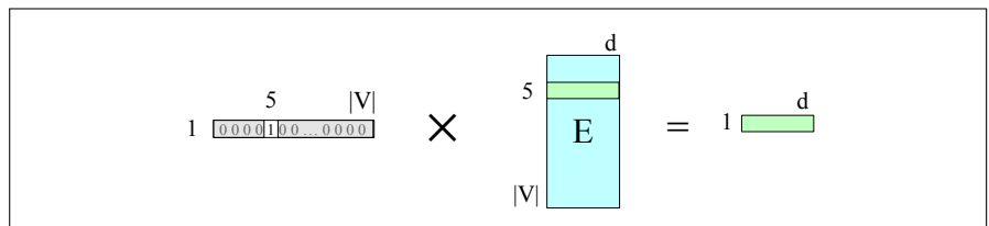
Figure 9.11 Selecting the embedding vector for word V_5 by multiplying the embedding matrix \mathbf{E} with a one-hot vector with a 1 in index 5.
