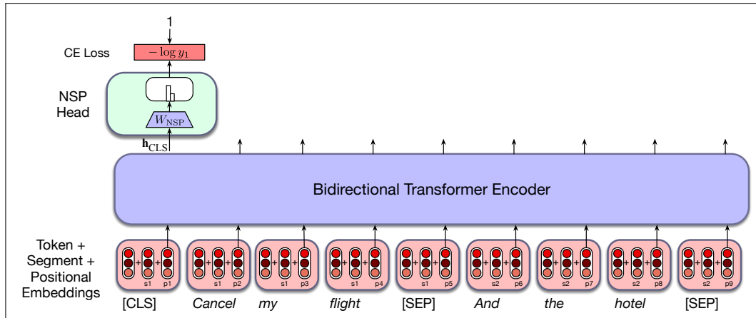
Figure 11.4 An example of the NSP loss calculation.
