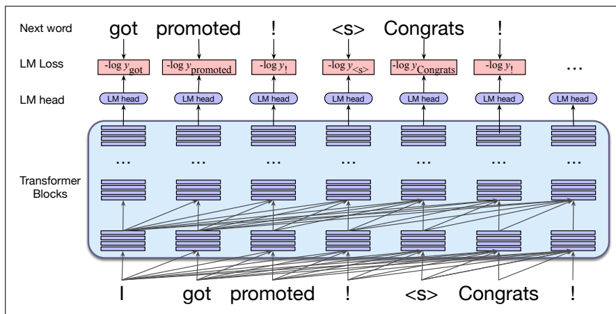
Figure 15.13 Training a causal (decoder-only) language model for a chatbot.
