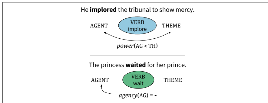
Figure 22.15 The connotation frames of Sap et al. (2017), showing that the verb implore implies the agent has lower power than the theme (in contrast, say, with a verb like demanded ), and showing the low level of agency of the subject of waited . Figure from Sap et al. (2017).
