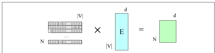
Figure 9.12 Selecting the embedding matrix for the input sequence of token ids W by multiplying a one-hot matrix corresponding to W by the embedding matrix \mathbf{E} .
