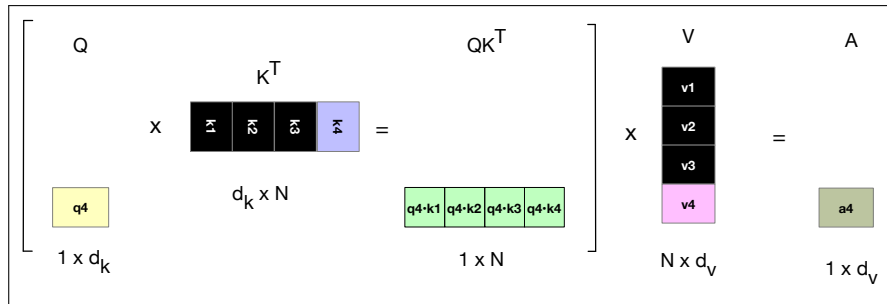
Figure 10.7 Parts of the attention computation (extracted from Fig. 9.10) showing, in black, the vectors that can be stored in the cache rather than recomputed when computing the attention score for the 4th token.
