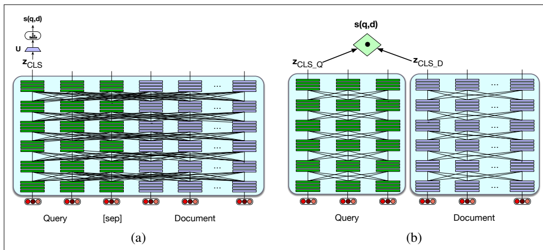
Figure 14.7 Two ways to do dense retrieval, illustrated by using lines between layers to schematically represent self-attention: (a) Use a single encoder to jointly encode query and document and finetune to produce a relevance score with a linear layer over the CLS token. This is too compute-expensive to use except in rescoring (b) Use separate encoders for query and document, and use the dot product between CLS token outputs for the query and document as the score. This is less compute-expensive, but not as accurate.
