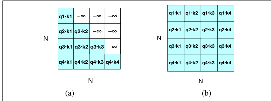
Figure 11.2 The N \times N \mathbf{QK}^T matrix showing the q_i \cdot k_j values, with the upper-triangular portion of the comparisons matrix zeroed out (set to -\infty , which the softmax will turn to zero).
